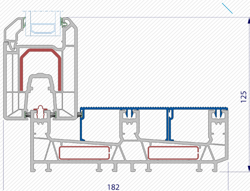
Cill Section
