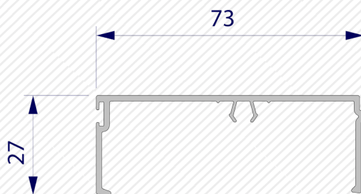
4457 (triple track PVC trim)
